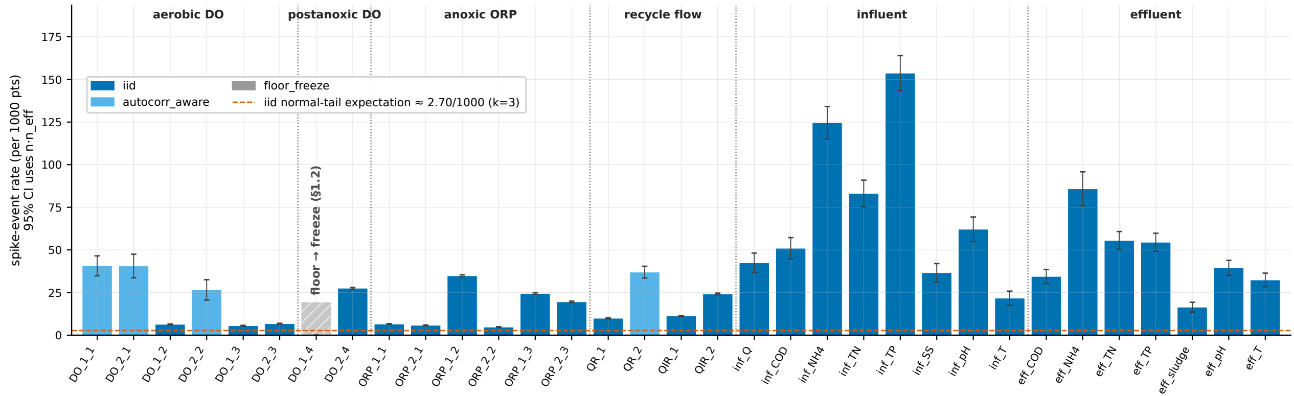
Figure A3. Whitening sanity check — local-Hampel spike-event RATE (per 1000 pts; manifest-keyed input; formal detection → §1.2 D1)
